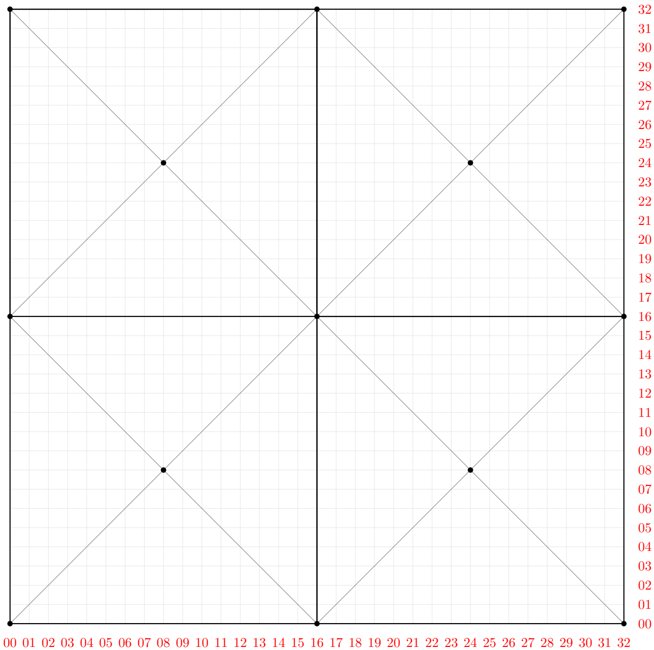
Level 0 Balanced Tree
