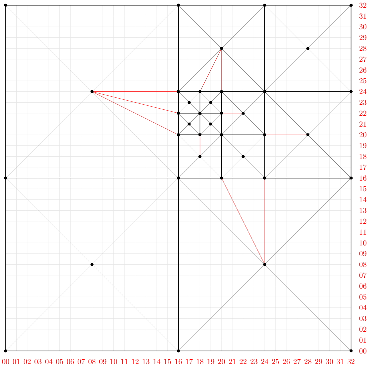
Level 3 Balanced Tree
